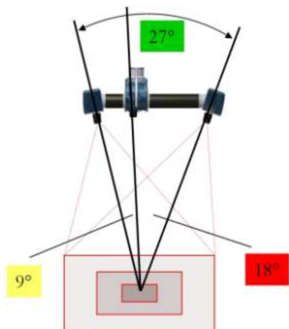
Figure 2: Asymmetrical 2-camera setup.
